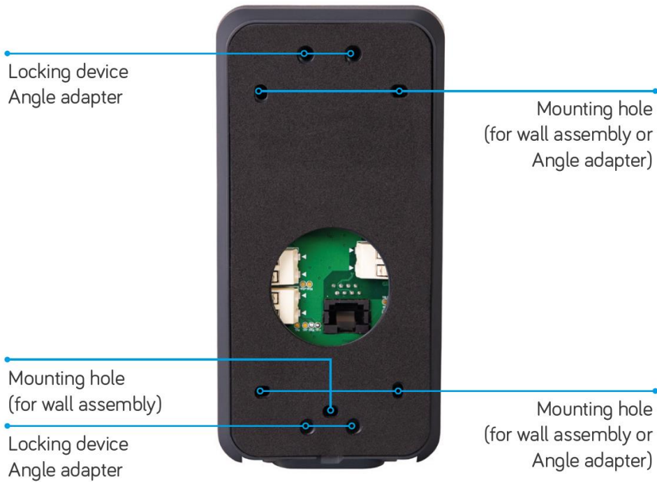
Figure 2: Rear view
