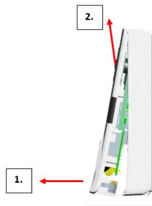
Figure 15: Removing the upper part of the housing
