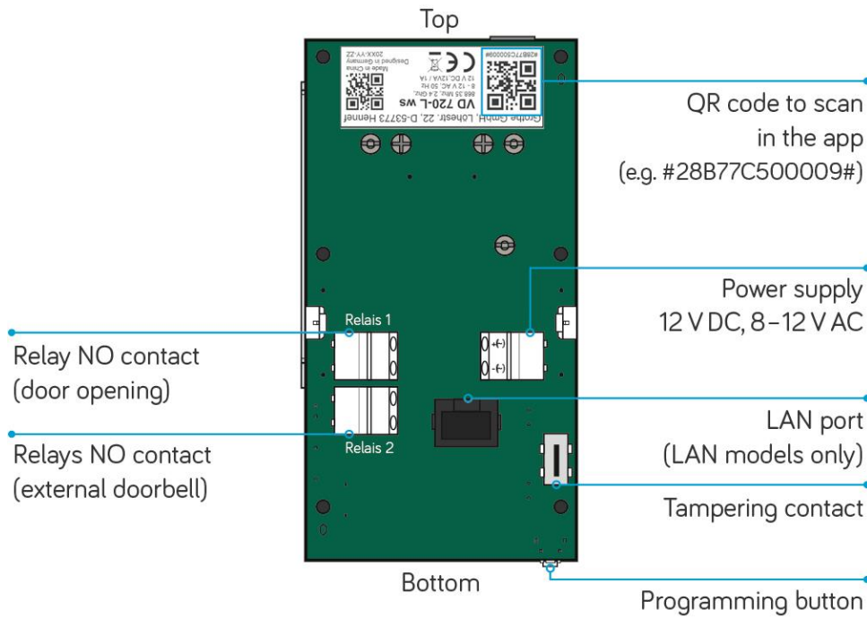
Figure 4: Overview circuit board
