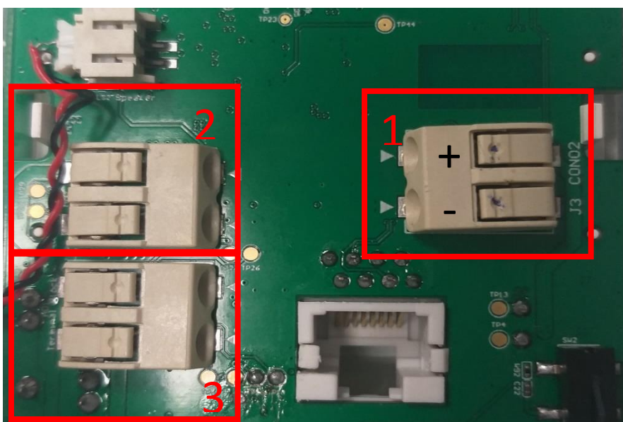
Figure 5: Electrical connections
