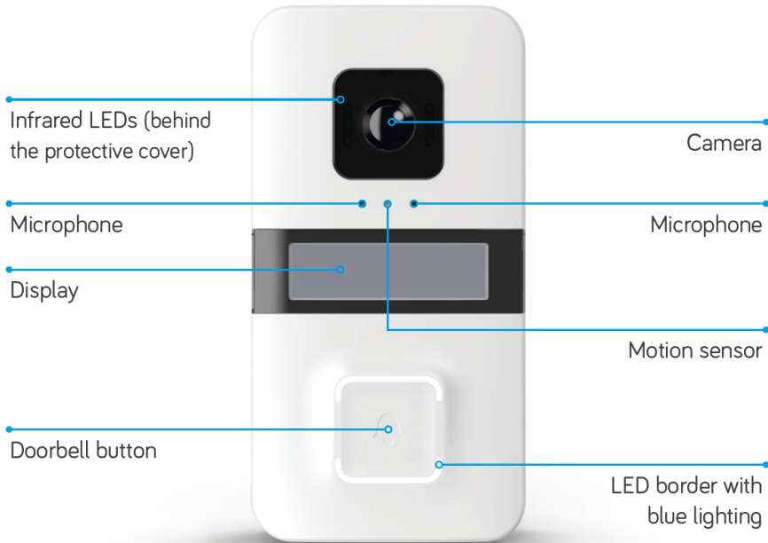
Figure 1: Front view
